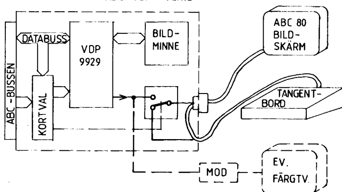
BLOCKSHEMA ABC-VDP VER.2
